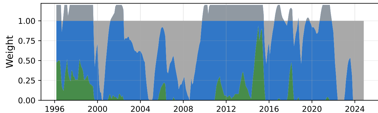
Transaction cost 0.0005 Sharpe 0.61; turn 99%
