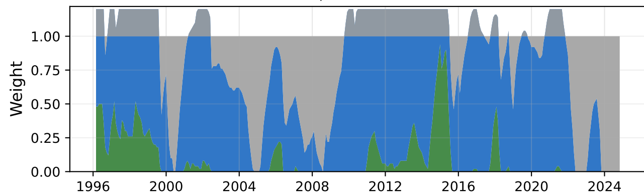
Transaction cost 0.0025 Sharpe 0.56; turn 98%
