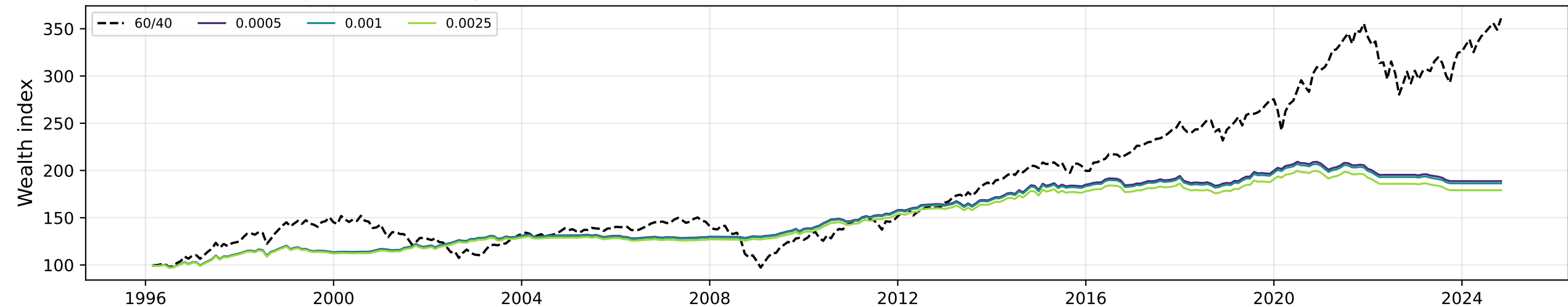
Transaction cost 0.0005 Sharpe 0.61; turn 99%
